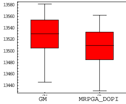
(a) 50 runs, n=100 , k=200
