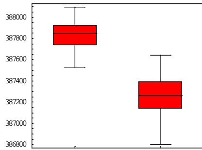
(c) 50 runs, n=3000 , k=200
