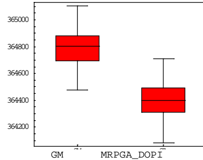
(b) 50 runs, n=100 , k=5000
