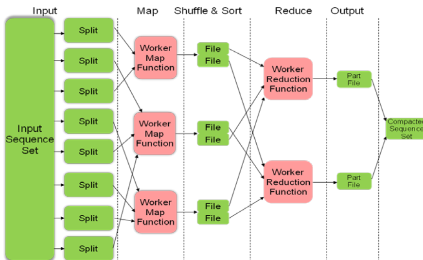
Fig. 2. MapReduce Dataflow
