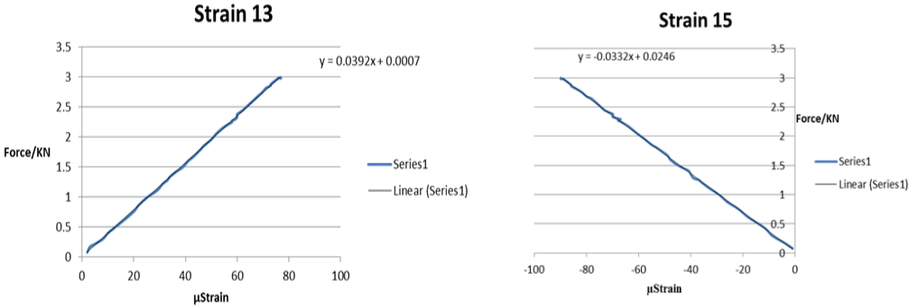
Figure 3: Force against Strain- Strain 13 and 15
