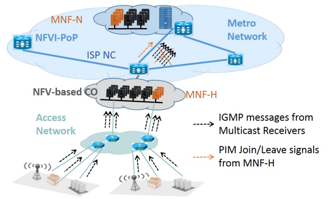
Fig. 2: Multicast Group Membership Management Analysis
