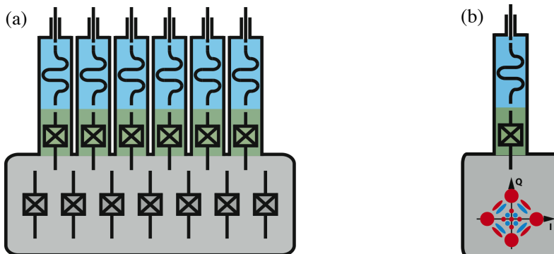
Figure 1: (a) A protected logical qubit consisting of a register of many qubits: here, we see a possible architecture for the Steane code [11] consisting of 7 qubits requiring the measurement of 6 error syndromes. In this sketch, 7 transmon qubits in a high-Q resonator and the measurement of the 6 error syndromes is ensured through 6 additional ancillary qubits with the possibility of individual readout of the ancillary qubits via independent low-Q resonators. (b) Minimal architecture for a protected logical qubit, adapted to circuit quantum electrodynamics experiments. Quantum information is encoded in a Schrödinger cat state of a single high-Q resonator mode and a single error syndrome is measured, using a single ancillary transmon qubit and the associated readout low-Q resonator.
