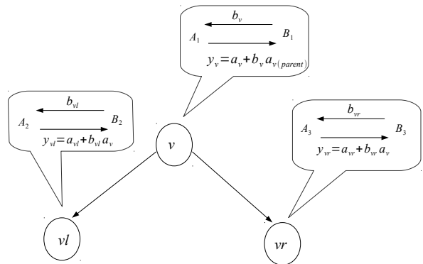
Figure 1: Pictorial view for an internal node of the Tree protocol. Here the coloring is such that c(v) = 1, c(v\ell) = 2, c(vr) = 3 .
