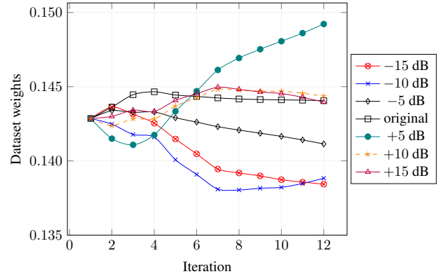
Fig. 2: Data weights learned using simulated+real development data. The sum of the weights is normalized to 1.
