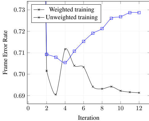
Fig. 1: FER on the development set achieved by weighted vs. unweighted training using simulated+real development data. The FER equals 0.999 for both systems at iteration 1.
