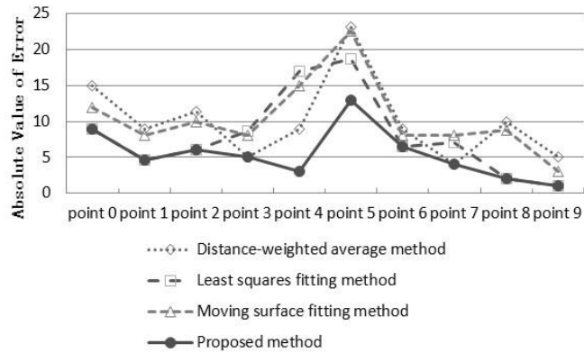
Fig. 3. Absolute value of error in glacier areas
