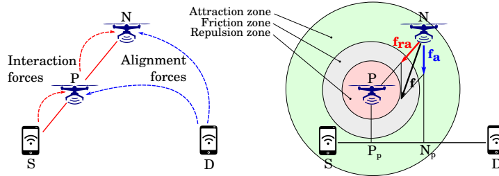
Fig. 2. (left) Principles of virtual forces applied on nodes P and N in a communication chain, (right) detailed forces on N (note that friction \mathbf{f}_{fr} is non-existent in this case).
