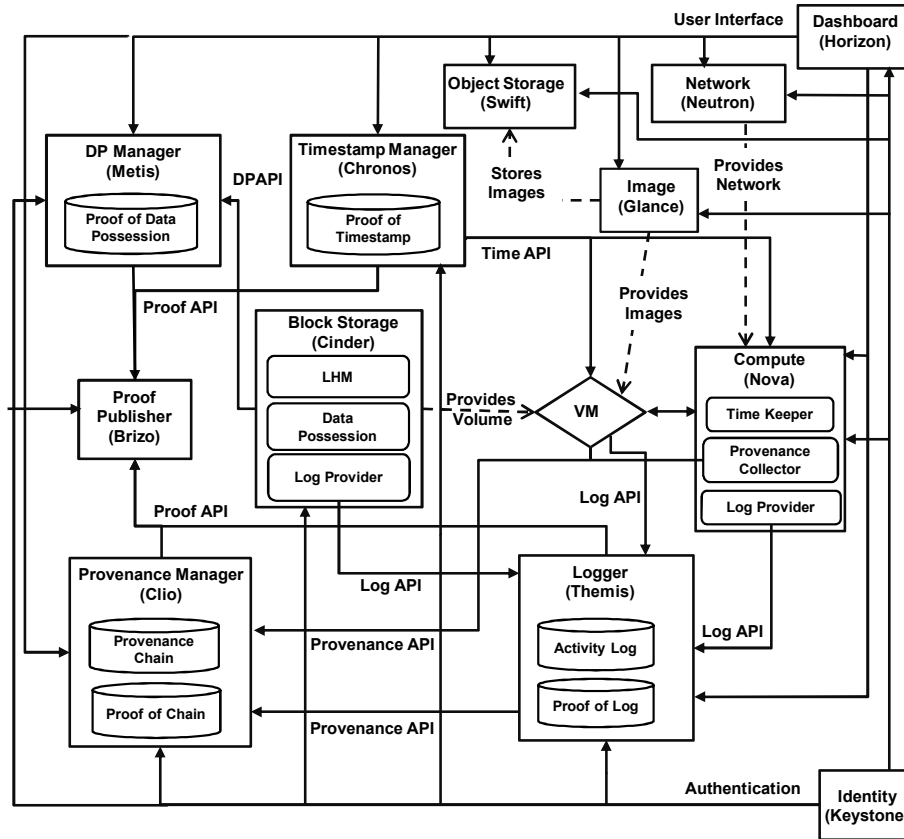
Figure 1. FECloud architecture.
