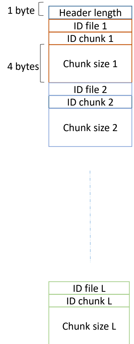
c) header structure
