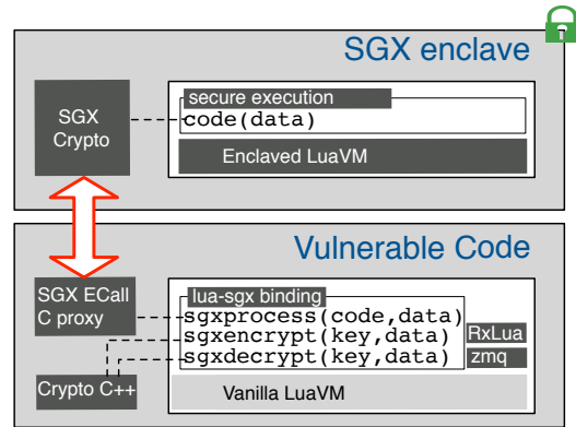
Figure 3: Integration between LUA and Intel® SGX.
