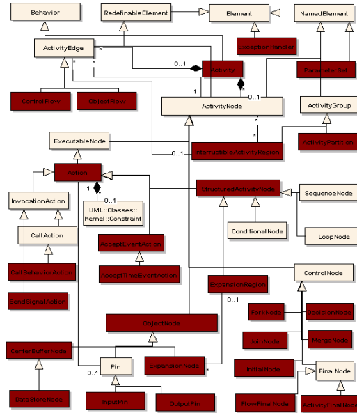
Figure 1. UML-AD meta-model
