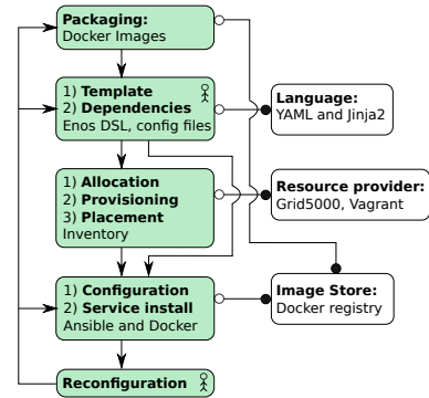
Fig. 3. Enos model
