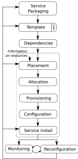
Fig. 1. Deployment model
