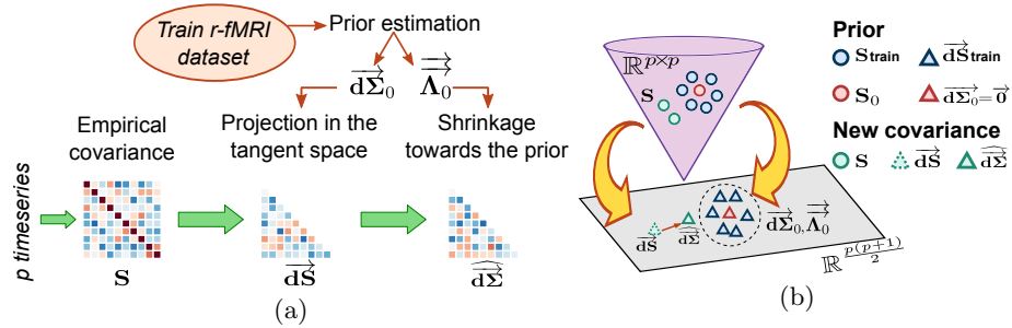
Fig. 1. (a) Shrank embedding estimation workflow: the empirical covariance is estimated from r-fMRI time-series; it is projected onto a tangent space built from a prior population; the embedding is then shrunk towards the prior ( \vec{d\Sigma}_0, \vec{\Lambda}_0 ). (b) Principle of tangent embedding shrinkage towards population distribution.
