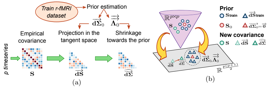
Fig. 1. (a) Shrank embedding estimation workflow: the empirical covariance is estimated from r-fMRI time-series; it is projected onto a tangent space built from a prior population; the embedding is then shrunk towards the prior ( \vec{d\Sigma}_0, \vec{\Lambda}_0 ). (b) Principle of tangent embedding shrinkage towards population distribution.
