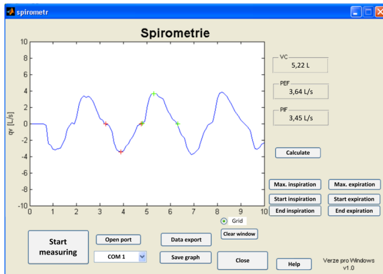
Fig. 2. Software window.
