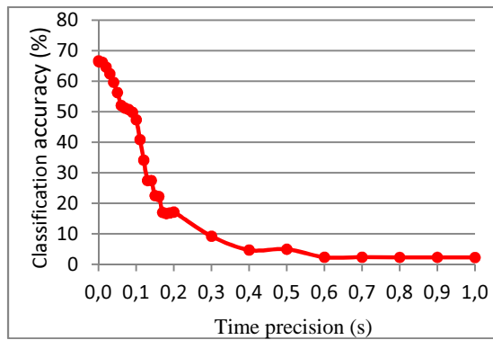
Fig. 5. Influence of time precision on algorithm's classification accuracy
