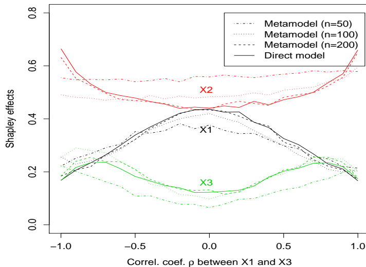
Figure 7: Sensitivity indices on the Ishigami function estimated by 3 metamodels built on 3 different learning databases. The exact permutation method (with N_o = 2 \times 10^3 , N_i = 3 , N_v = 10^4 ) is applied on the metamodel predictor.
