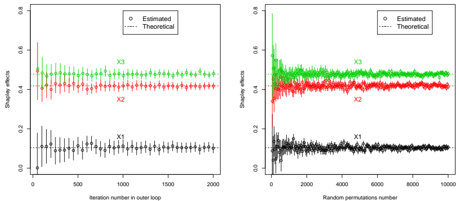
Figure 5: Numerical estimates by the exact permutation method (a) and the random permutation method (b) of the Shapley effects on the linear model.
