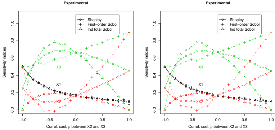
Figure 6: Numerical estimation of sensitivity indices on the linear model. Left: exact permutation method ( N_o = 5 \times 10^3 , N_i = 3 , N_v = 10^4 ). Right: random permutation method ( m = 3 \times 10^4 , N_o = 1 , N_i = 3 , N_v = 10^4 ).
