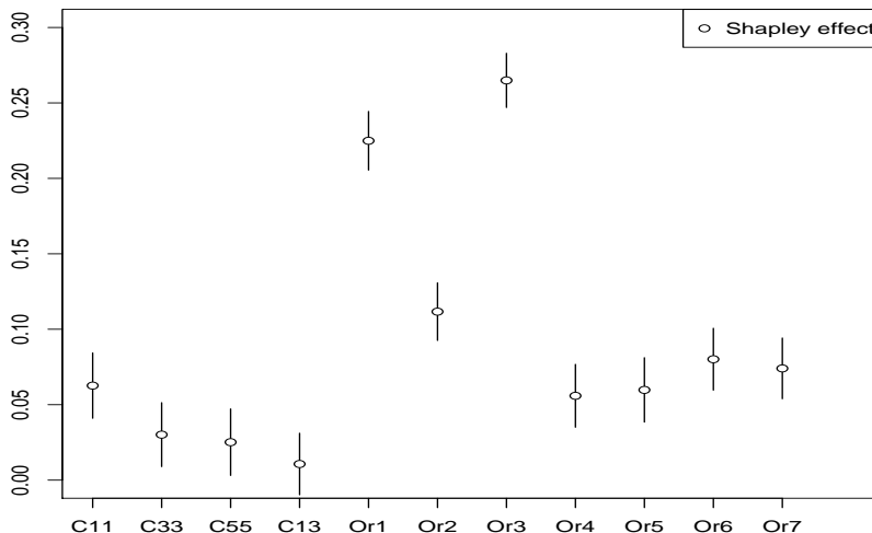
Figure 9: Shapley effects for the ultrasonic non-destructive control application. The vertical bars represent the 95%-confidence intervals of each effect.
