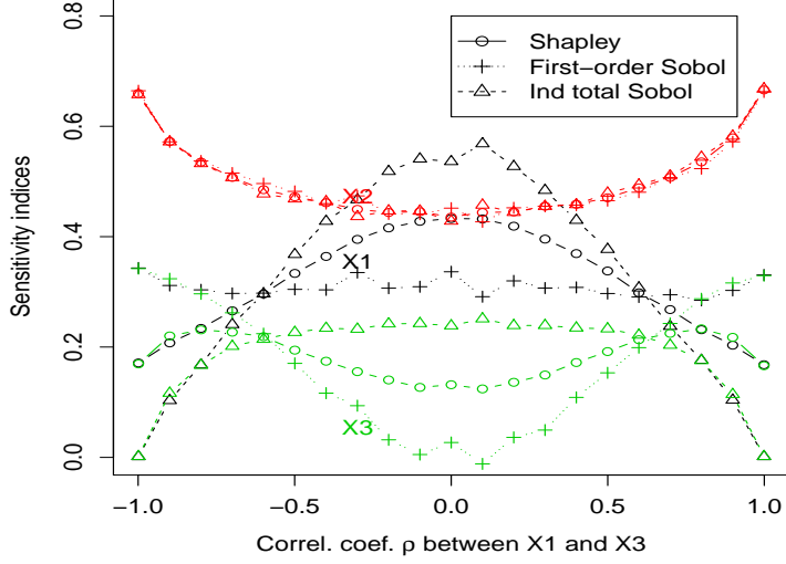
Figure 4: Sensitivity indices on the Ishigami function. Exact permutation method with N_o = 2 \times 10^4 , N_i = 3 , N_v = 10^4 .
