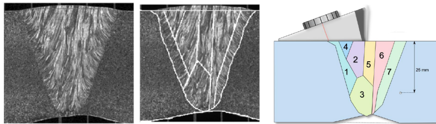
Figure 8: Metallographic picture (left), description of the weld in 7 homogeneous domains (middle) and inspection configuration (right). From [48].
