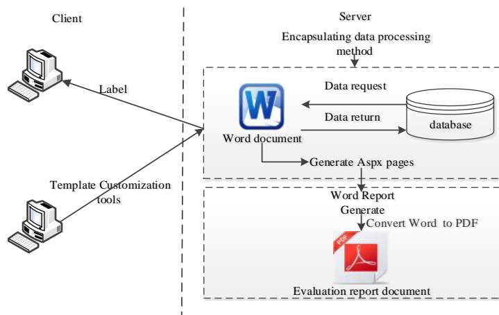
Figure 1 The structure of Evaluation report generation module
