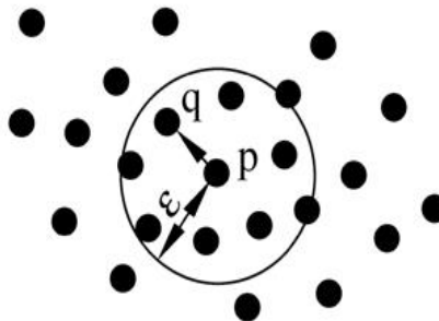
Figure 3. Directly density-reachable
