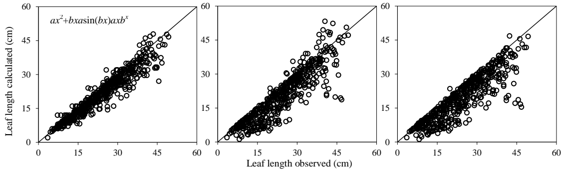
Fig. 4. Comparison of the observed and the simulated leaf length on main stem in 2011-2012
