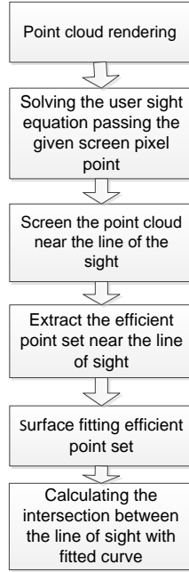
Fig.1. The algorithm flow of the mapping from the screen pixel point to the object surface coordinate point
