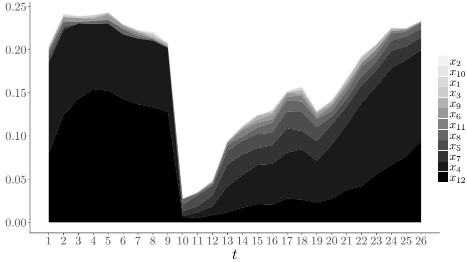
Figure 6: Cumulative area plot of first-order Sobol' index estimates for the levelE model. The y-axis indicates the sum of the estimates. The x-axis refers to the time frame t .
