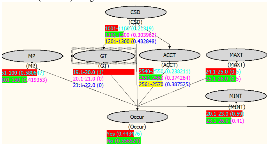
Fig. 5. Reverse reasoning
