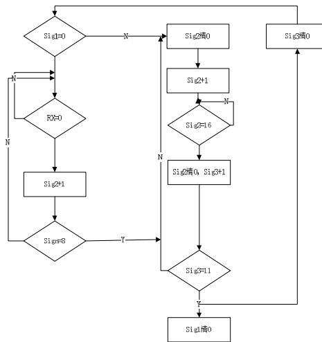
Figure 12 Flow Chart of Asynchronous Receiving Module
