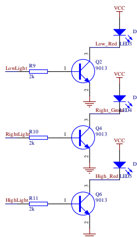
Figure 6 Position-Pilot-Lamp-Driving Circuit
