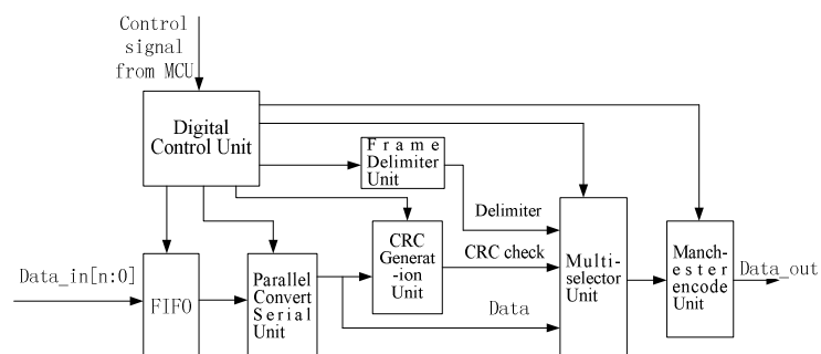
Fig. 2. Encoder architecture
