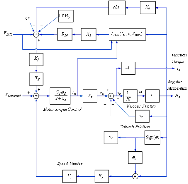
Fig.1. High Fidelity Reaction Wheel Block Diagram
