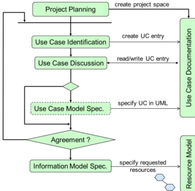
Fig. 5. Analysis phase of the SERVUS Methodology
