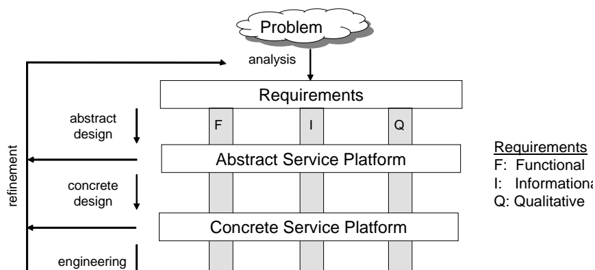
Fig. 2. Analysis, Design and Engineering Steps [3]
