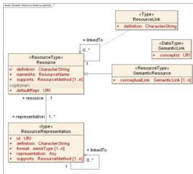
Fig. 3. SERVUS Semantic Resource Model [3]
