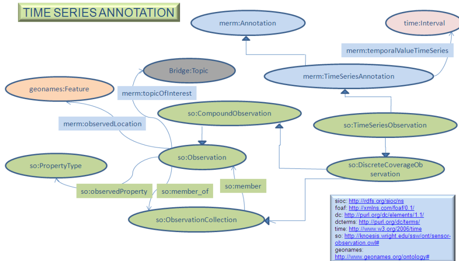
Fig. 4. TimeSeriesAnnotation model
