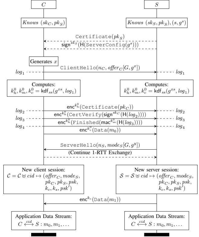
Figure 3: DH-based 0-RTT in TLS 1.3 Draft-12, inspired by QUIC and OPTLS.
