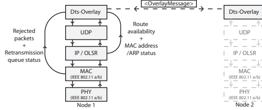
Fig. 1. Cross-layer Information Flow in Dts-Overlay.
