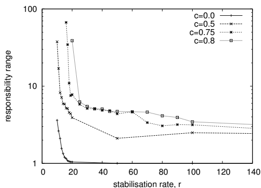
Fig. 3. Responsibility range as function of stabilisation rate for various values of c . Even for low churn, NATs introduce a large amount of lookup inconsistencies as indicated by the range being greater than 1
