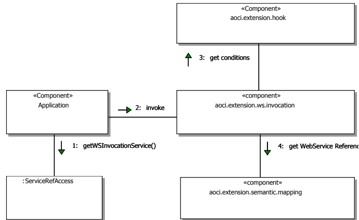
Fig. 8. Invocation phase
