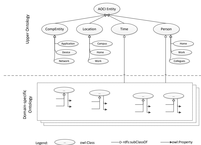
Fig. 2. Upper and domain-specific ontology
