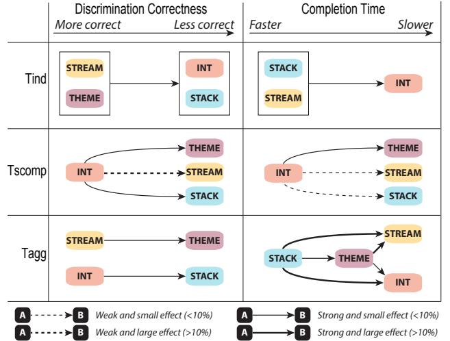
Figure 5: Summary of differences between techniques for discrimination correctness and completion time by task. In each cell, the horizontal position of each technique icon encodes its performance, ordered from best (left) to worst (right). Two icons with the same horizontal position mean that the two techniques perform similarly.
