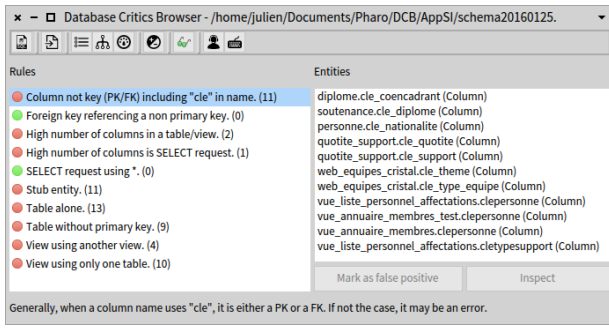
Fig. 1. The DBCritics GUI. Left panel: Rules that have been run on the model. Right panel: Entities violating the selected rule.
