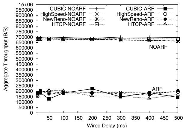
(a) 802.11b
