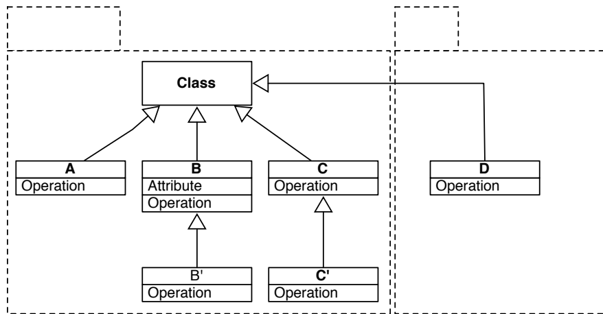
Figure 12-8 One single class vs. a nice hierarchy.
