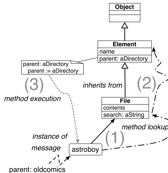
Figure 13-7 When an object receives a message, the corresponding method is looked up in its class and if necessary its superclasses (Step 1 and 2). Then the method is executed on the message receiver (Step 3).
