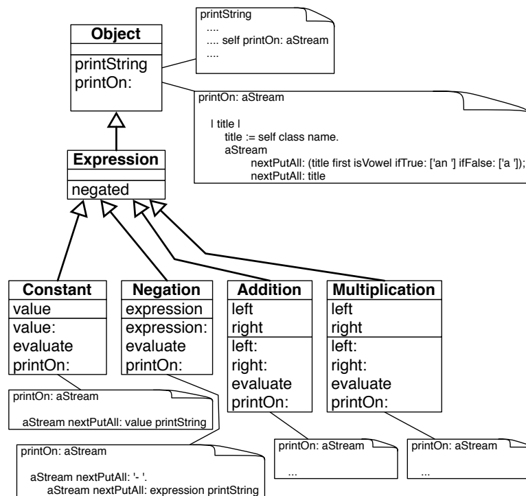
Figure 15-6 printOn: and printString a “hooks and template” in action.
