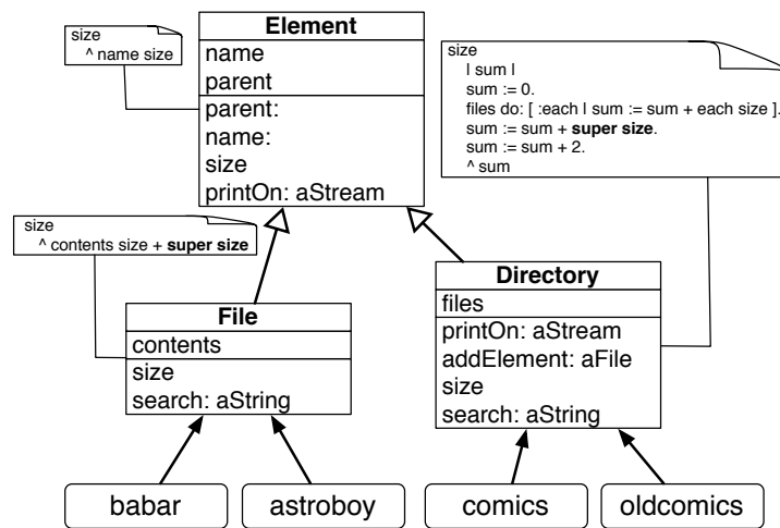
Figure 14-4 Using super to invoke the overridden method size.
