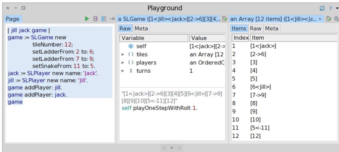
Figure 17-10 Playing step by step inside the inspector.
