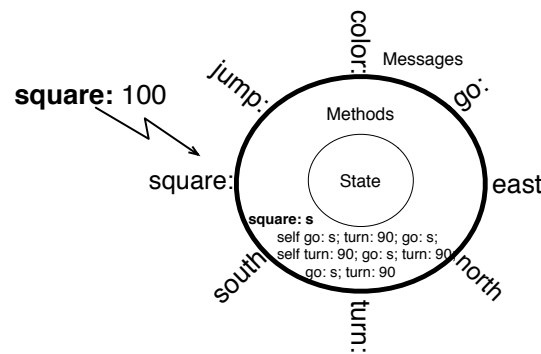
Figure 7-2 The message square: can be implemented differently. This different implementation does not impact the sender of the message who is not concerned by the internals of the object.
