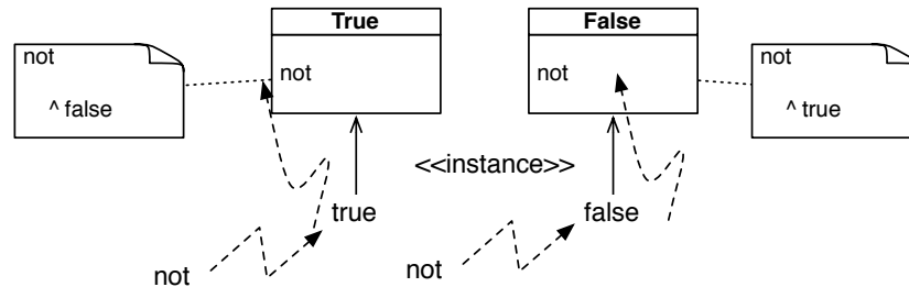
Figure 12-4 Sending a message selects the method in the class of the receiver.
