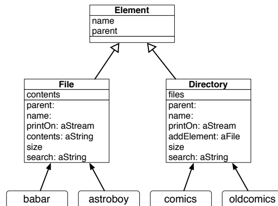
Figure 13-5 State factored between the two classes and their superclass.
