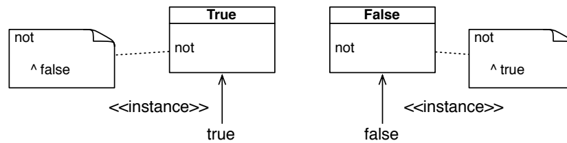
Figure 12-3 Two methods for one message each one returning the other instance.
