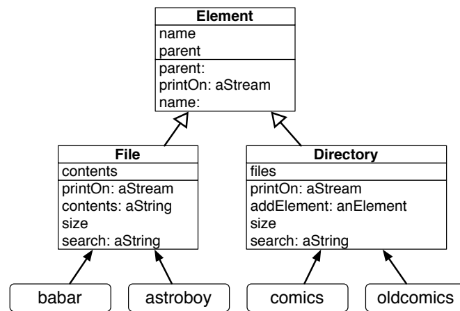
Figure 13-2 Two class taking advantages of inheriting from a common superclass.
