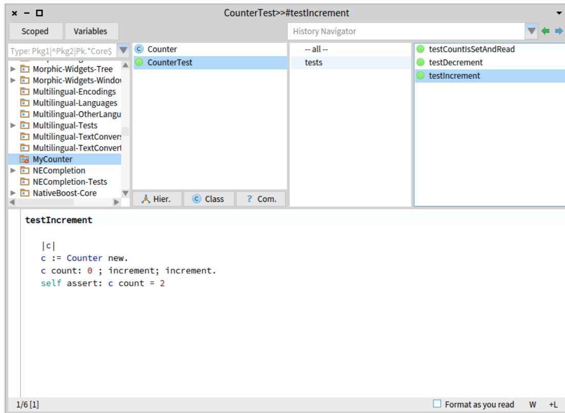
Figure 4-5 Class with green tests.
