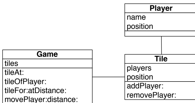
Figure 17-6 Current simple design: three classes with a player acting as a simple object.
