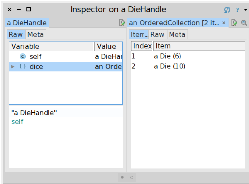
Figure 11-6 A die handle with more information.
