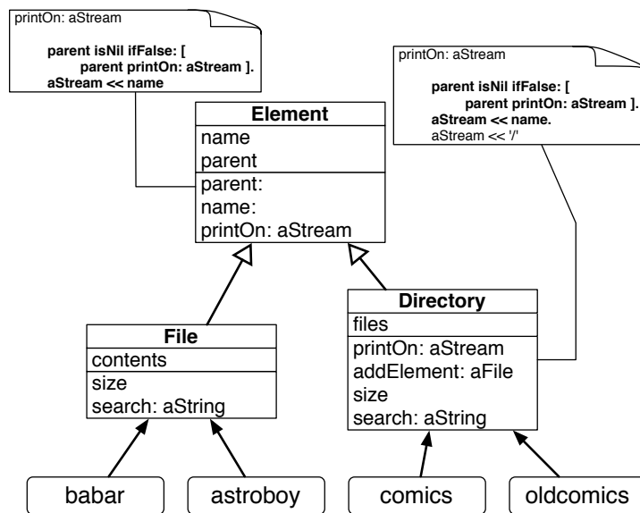
Figure 14-2 Improving the logic (but not fully).
