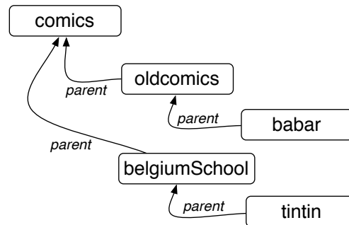
Figure 8-5 A graph of objects to represent our file system.
