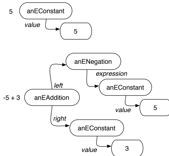
Figure 15-2 Expressions are composed of trees.
