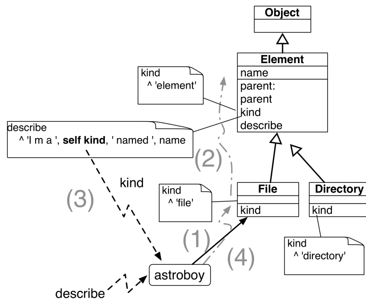
Figure 13-8 A self-send creates a hook (kind) that subclasses override. The method describe is called a template because it creates a context.
