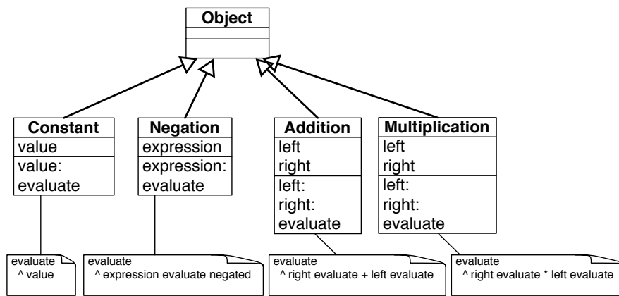
Figure 15-3 Evaluation: one message and multiple method implementations.
