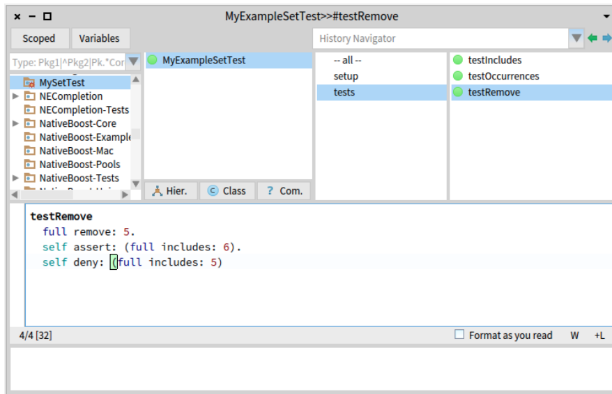
Figure 5-1 Running SUnit tests from the System Browser.
