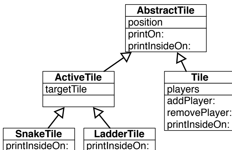
Figure 17-8 Introducing printInsideOn: as a new hook.
