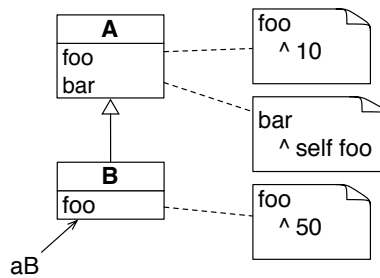
Figure 13-9 Self semantics abstractly explained.
