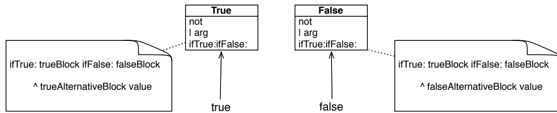
Figure 12-6 Conditional implementation: again two methods and no explicit tests.
