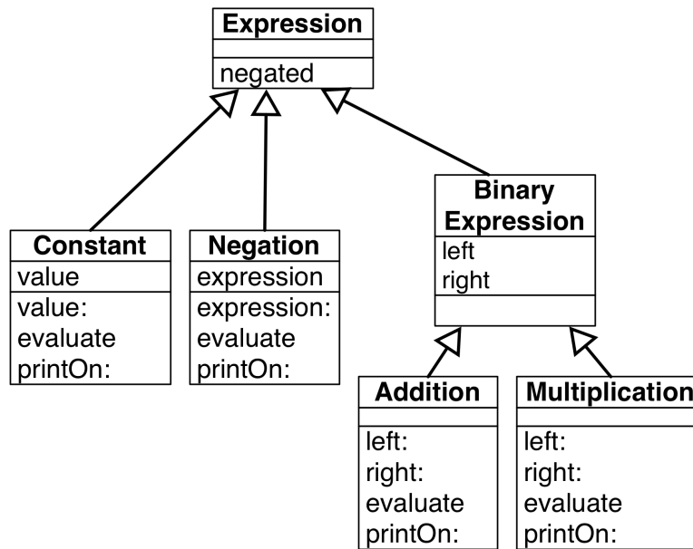
Figure 15-8 Factoring instance variables.
