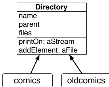
Figure 8-3 The Directory class and some instances (directories).
