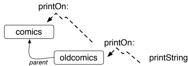
Figure 8-4 Navigating an object graph by sending message to different objects.
