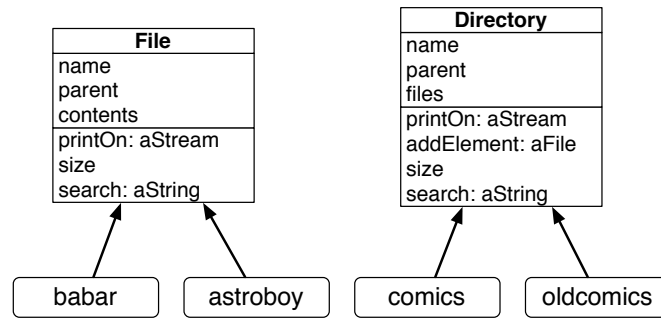
Figure 8-8 Two classes understanding similar sets of message.
