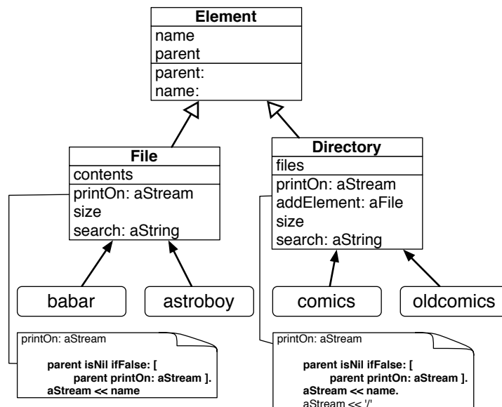
Figure 14-1 MFile and MDirectory contain duplicated logic in printOn: .
