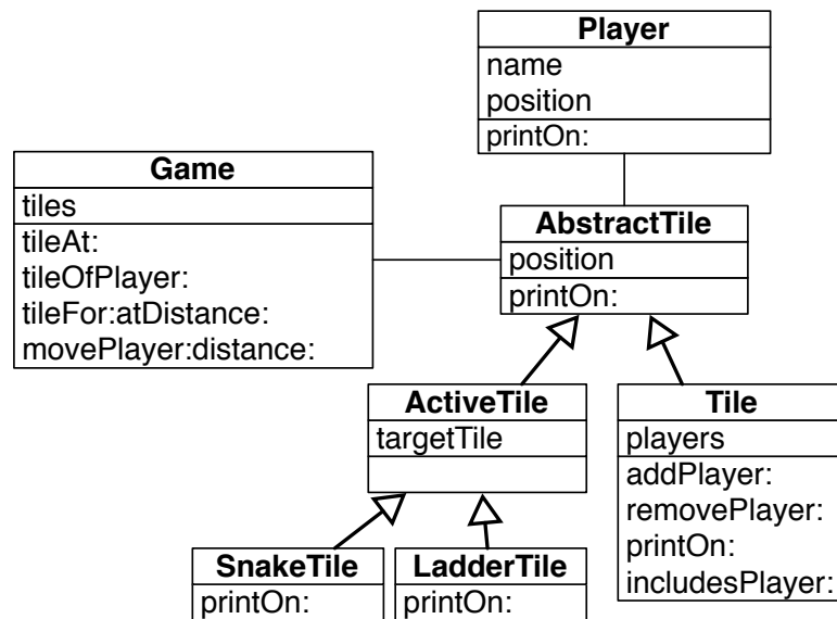
Figure 17-7 A hierarchy of tiles.
