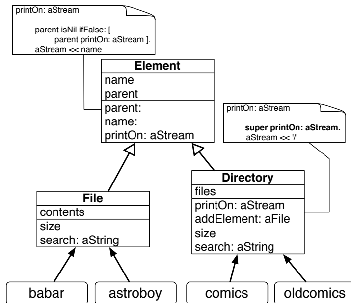
Figure 14-3 Using super to invoke the overridden method printOn: .
