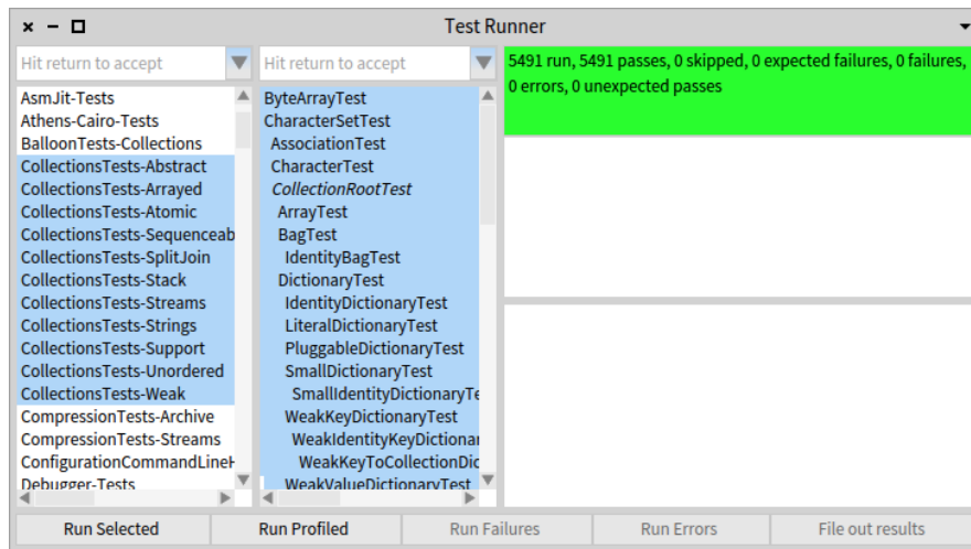
Figure 5-2 Running SUnit tests using the TestRunner .
