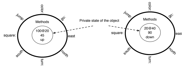
Figure 7-4 Two turtles have the same interface, i.e., set of messages being understood but they have different private state representing their direction, position and pen status.
