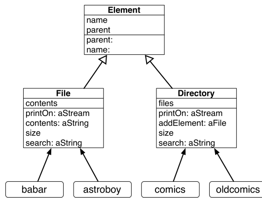
Figure 13-6 State and Methods factored out in the superclass.
