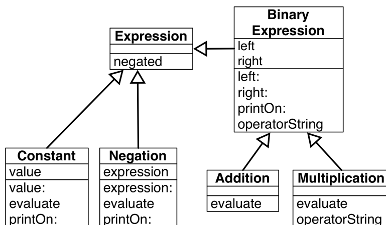
Figure 15-9 Factoring instance variables and behavior.
