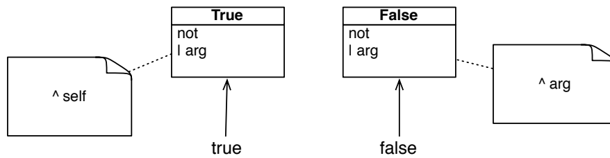
Figure 12-5 Disjunction implementation: two methods.
