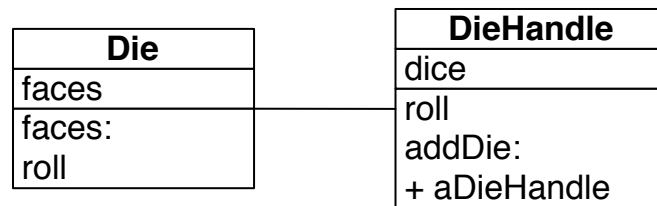
Figure 11-3 A die handle is composed of dice.
