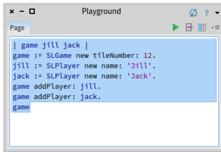
Figure 17-2 Playground in action. Use Do it and go - to get an embedded inspector.
