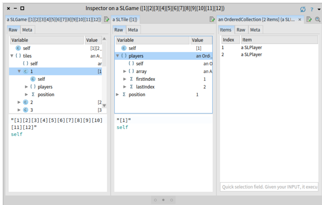
Figure 17-5 Navigating the objects using the navigation facilities of the inspector.
