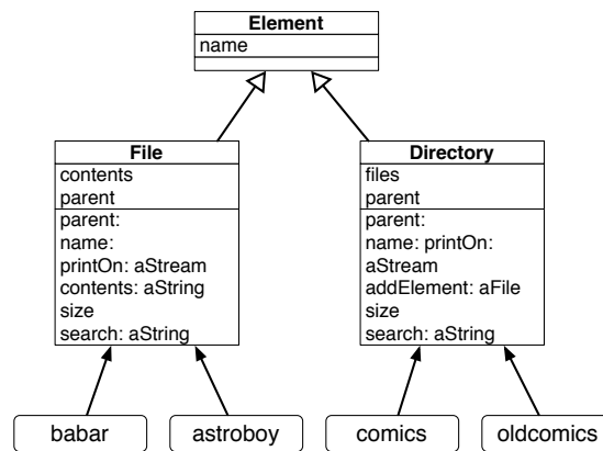
Figure 13-3 Moving the instance variable name to the superclass.
