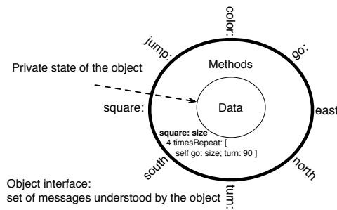
Figure 7-3 A turtle is an object which has an interface, i.e., a set of messages to which it can reply and a private state that only its methods can access.
