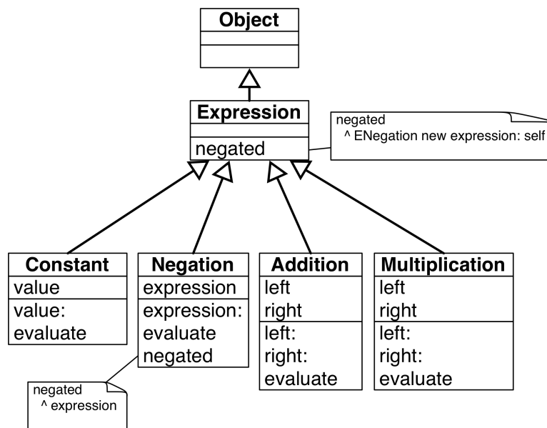
Figure 15-7 The message negated is overridden in the class ENegation .
