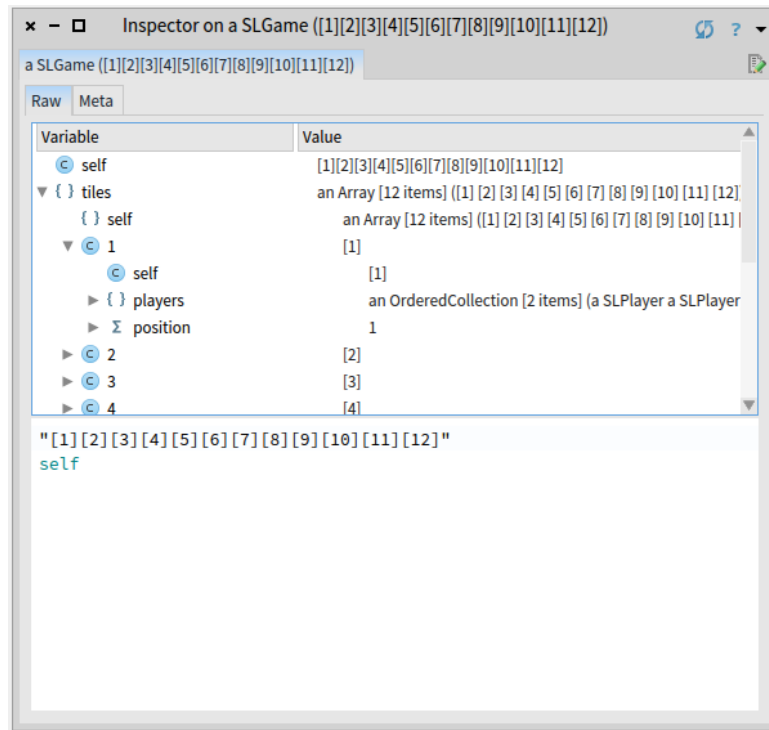
Figure 17-4 Navigating inside the game: getting inside the tiles and checking the players.
