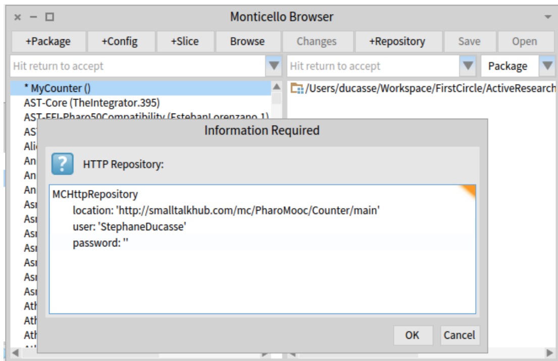
Figure 4-4 Editing the repository information.
