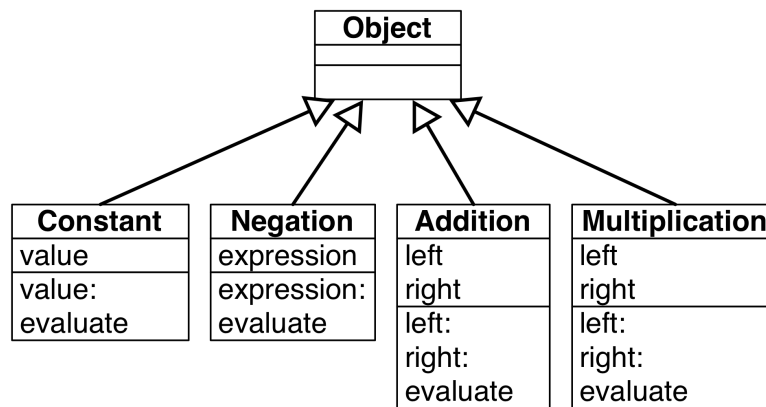
Figure 15-1 A flat collection of classes (with a suspect duplication).
