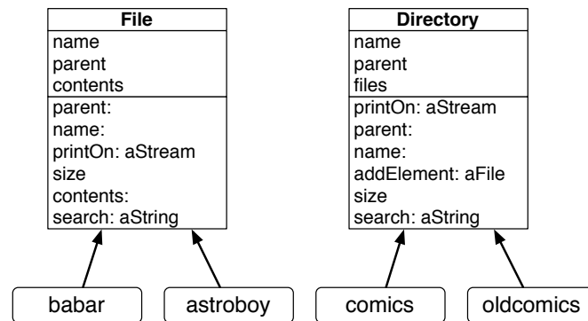
Figure 13-1 Two classes understanding similar sets of messages and structuring their instances in a similar way.
