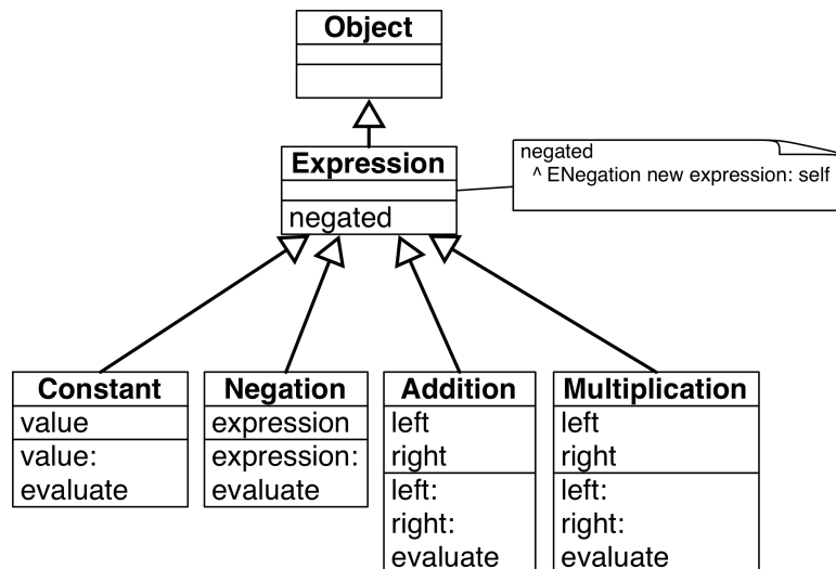
Figure 15-5 Introducing a common superclass.
