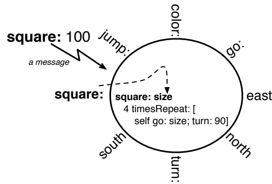
Figure 7-1 An object presents to the other objects an interface composed of a set of messages defining what he can do. This behavior is realized by methods that specify how the behavior is implemented. When a message is sent to an object a method with the message name (called selector) is looked up and executed.
