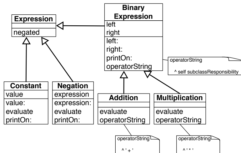
Figure 15-10 Better design: Declaring an abstract method as a way to document a hook method.
