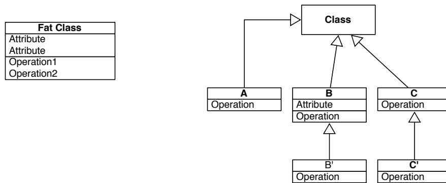
Figure 12-7 One single class vs. a nice hierarchy.
