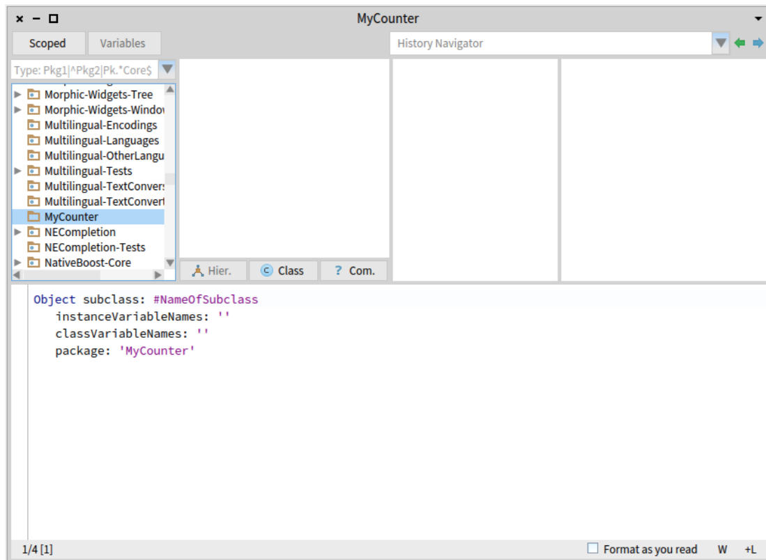
Figure 4-1 Package created and class creation template.
