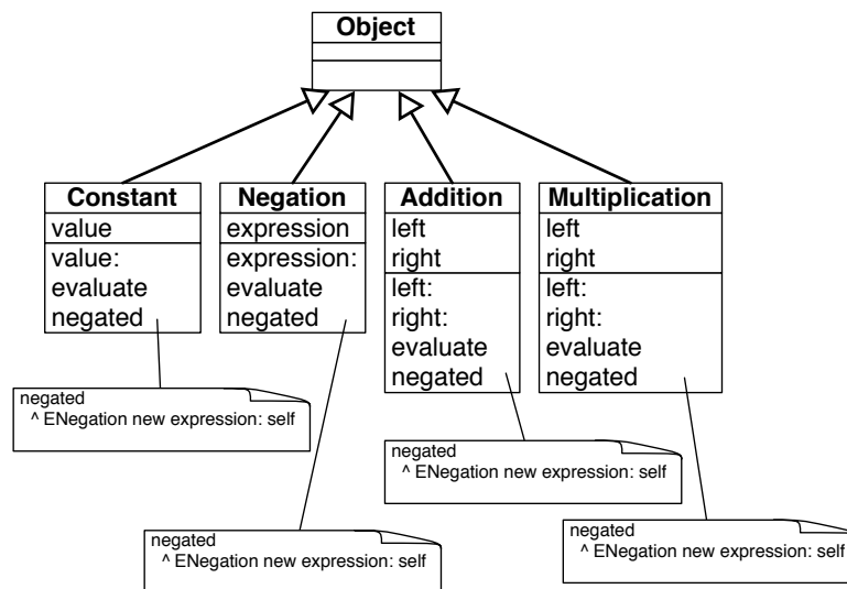
Figure 15-4 Code repetition is a bad smell.
