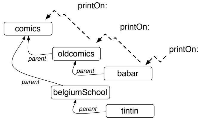
Figure 8-7 Printing a file: Sending messages inside a graph of different objects.
