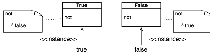
Figure 12-2 Two methods for one message.
