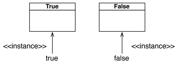
Figure 12-1 The two classes True and False and their respective unique instances true and false .
