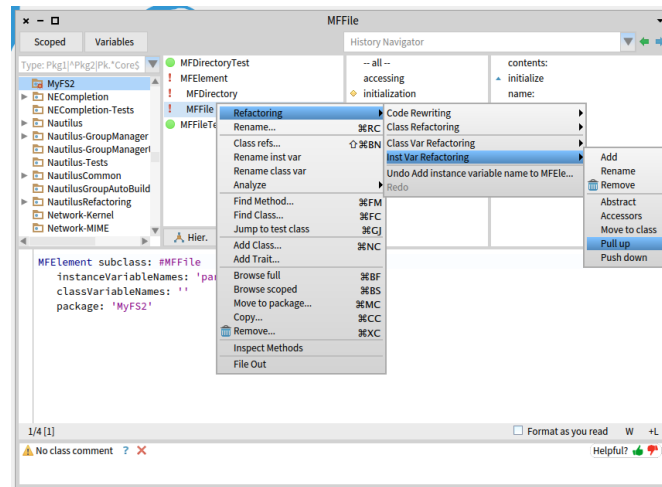
Figure 13-4 Applying the Pull Up Instance variable refactoring.
