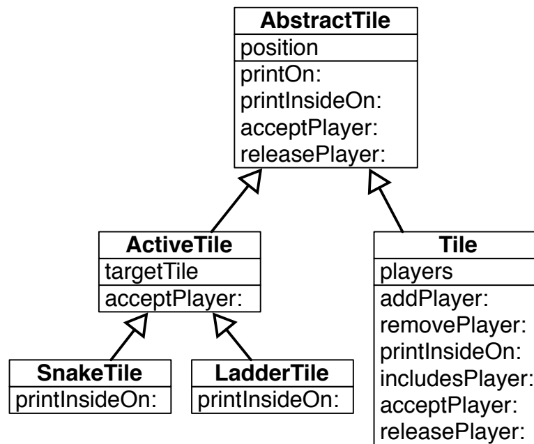
Figure 17-9 acceptPlayer: and releasePlayer: new message.
