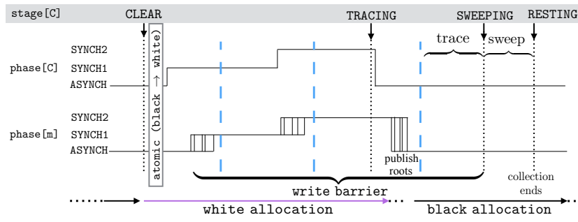
Figure 2: Timeline of a collection cycle. All mutators are coalesced into the bottom line, and the collector is shown in the top line. Dotted lines represent the GC start of a new stage, and dashed lines represent the end of a phase change (handshake).
