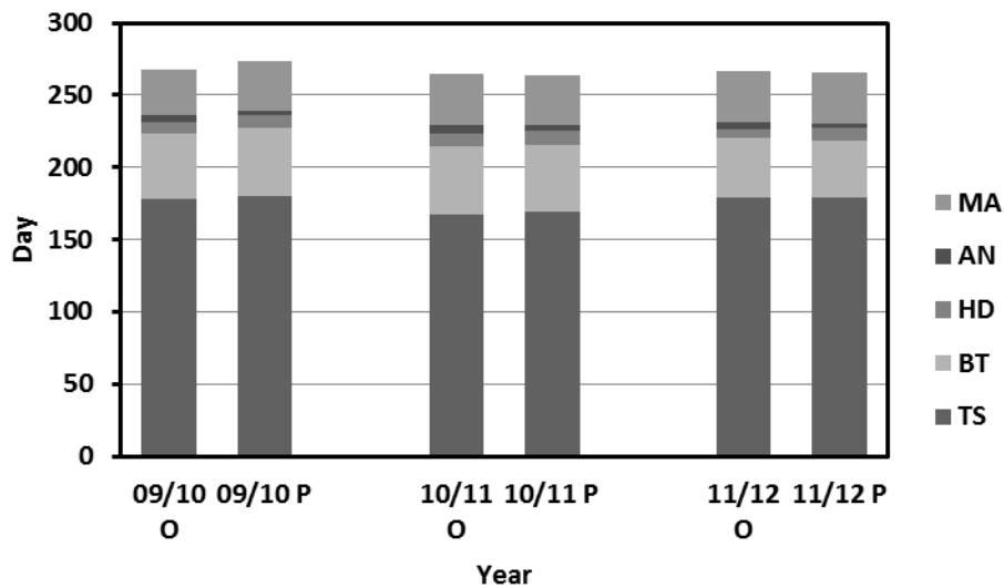
Fig. 3. Validation of observed (O) and predicted (P) day after planting (DAP) using the DSSAT-CERES model for TS, BT, HD, AN, MA in 3 growing seasons, 09/10, 10/11, 11/12 growing seasons.
