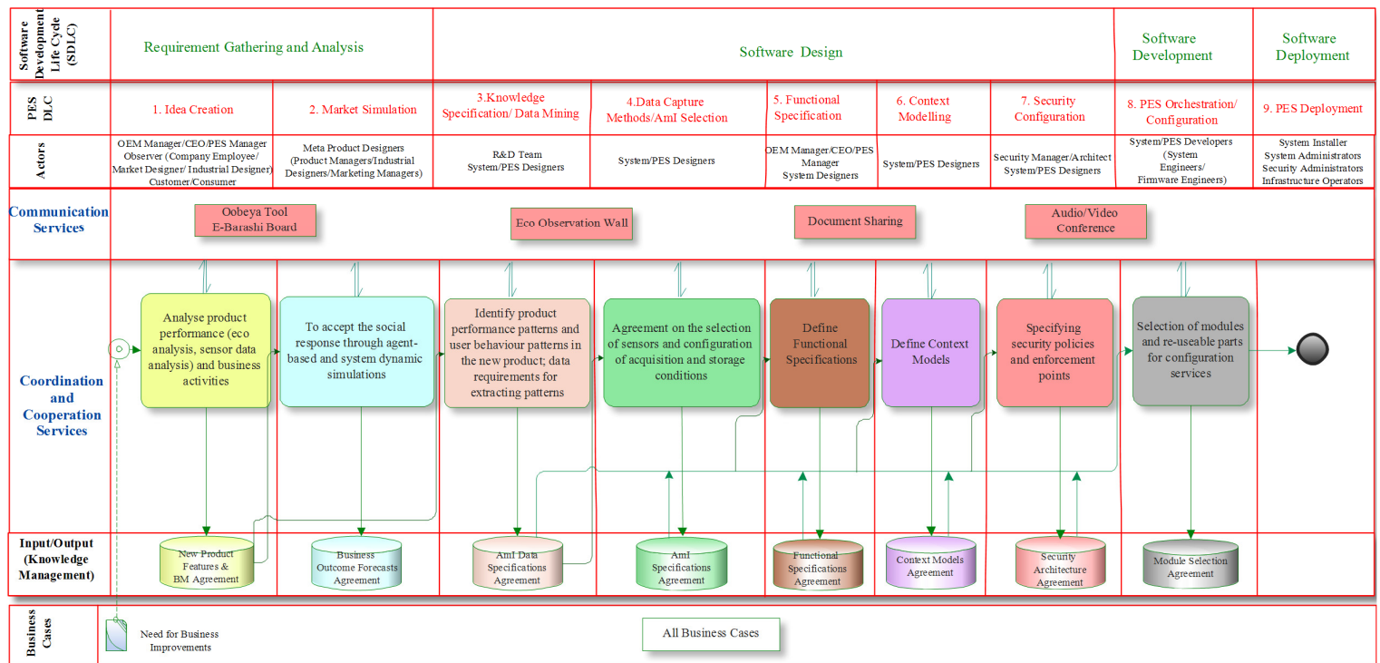
Fig. 1. The PES Collaborative Development Portal
