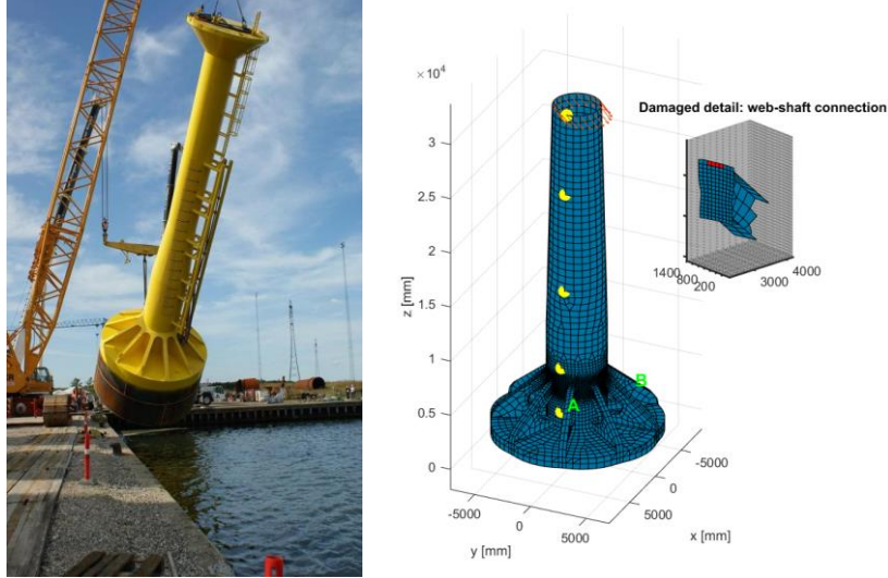
Fig. 1 MB foundation for a mobile met. mast at Horns Rev 2 (2009) (left). FE-model of the MB for numerical simulations (right). Bi-axial x-y accelerometers are illustrated by yellow dots.
