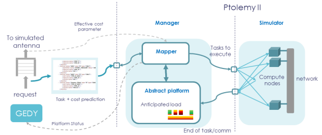
Figure 1: Simulation environment
