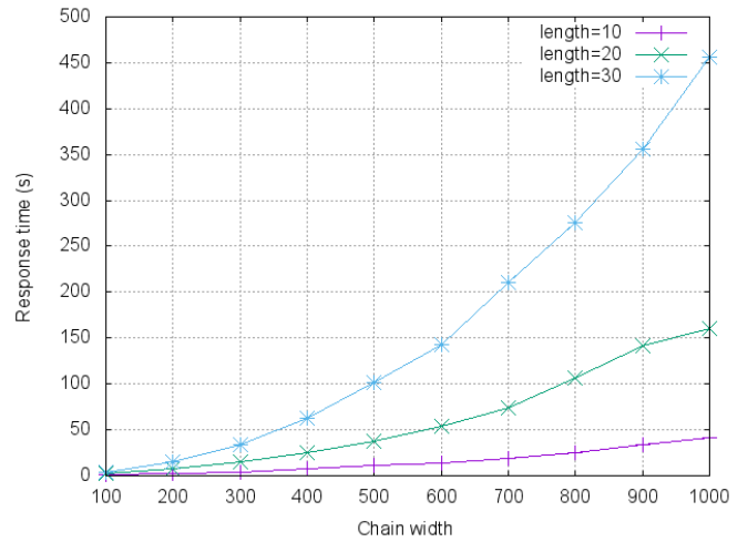
Figure 10. Response times of nuXmv vs. both width and length.
