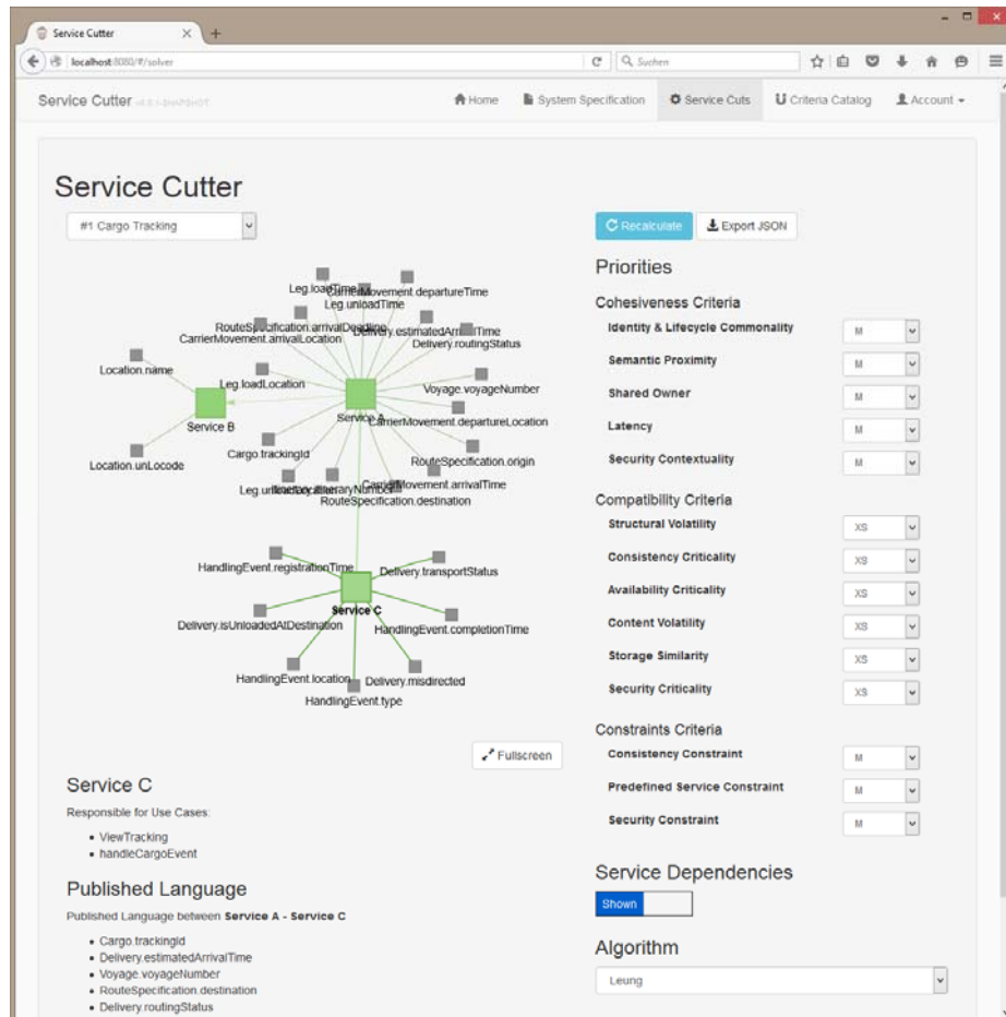
Figure 6. Screenshot of Service Cutter presenting a candidate service cut.
