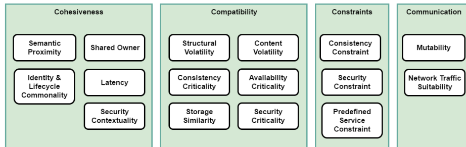
Figure 2. Coupling Criteria (CC) catalog compiling 16 CC in four categories.
