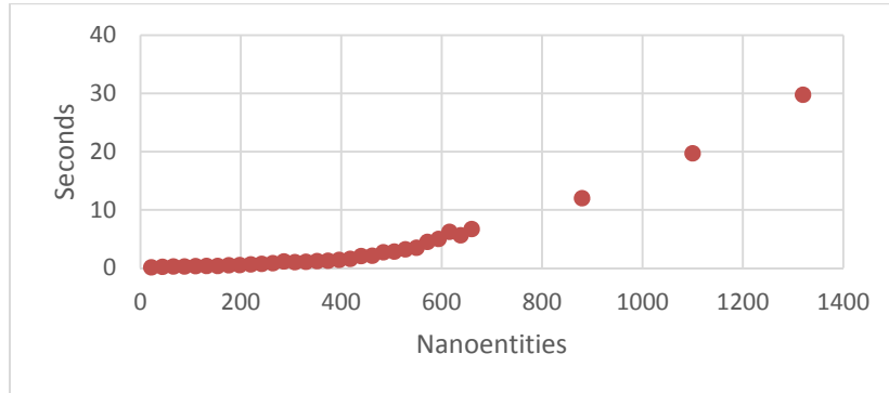
Figure 7. Performance test results: service cut calculation (scaled up sample application)
