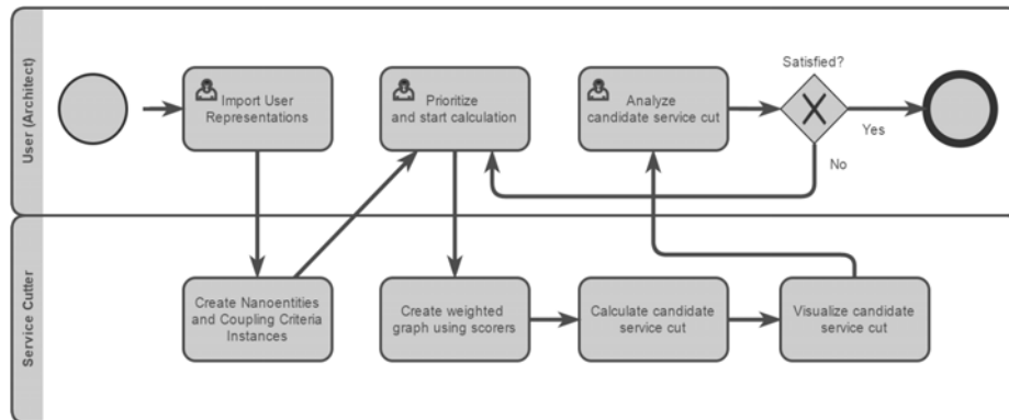
Figure 4. Serving decomposition process (human vs. automated/tool-supported tasks).
