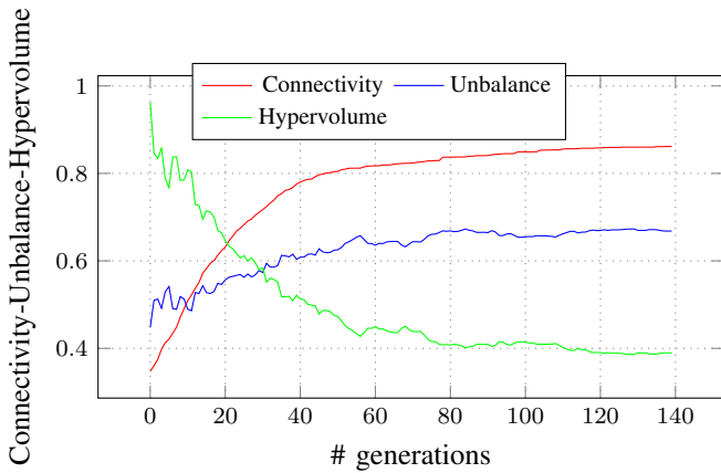
Fig. 5: Evolution along 150 generations - Mutation only GA
