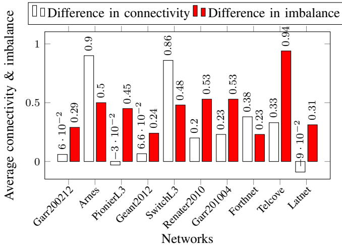
Fig. 3: Comparison Kmean/GA
