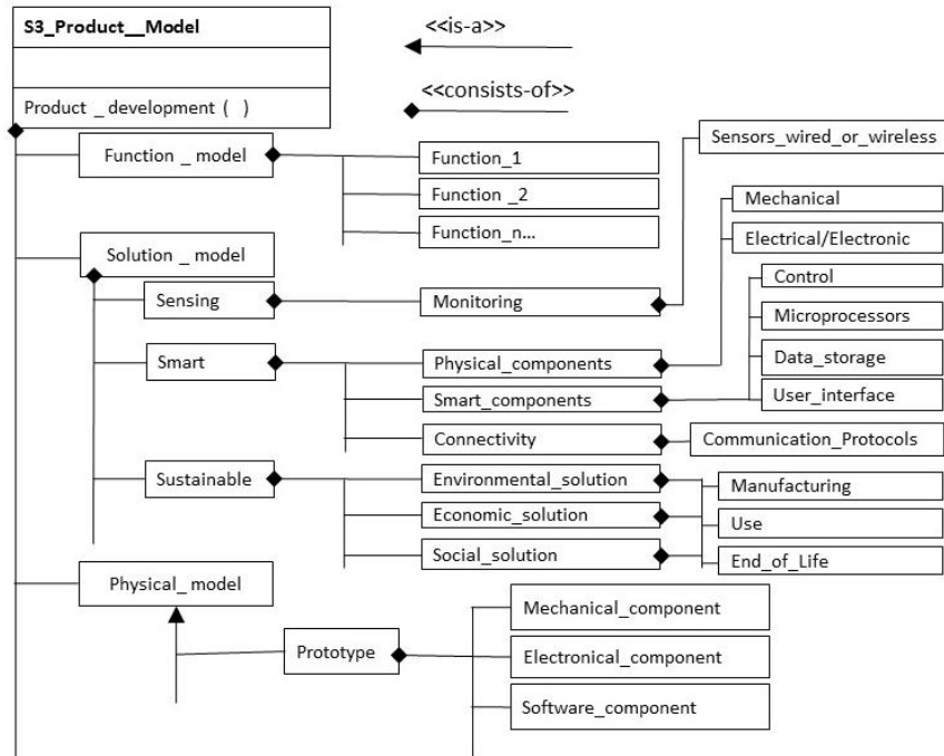
Fig. 3. Sensing, Smart and Sustainable Product Model [7]
