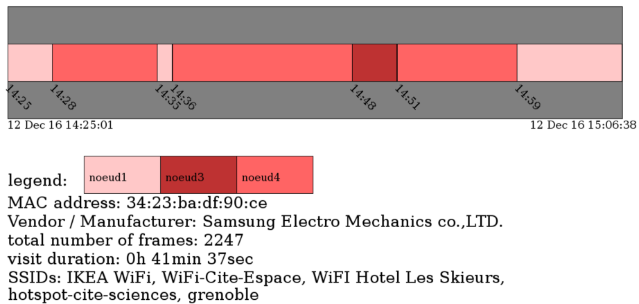
Figure 2: Basic user interface of Wombat displaying the device's MAC address, the list of SSIDs, as well as a mobility trace under a timeline form.
