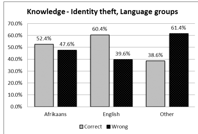
Figure 1. Vocabulary-type question
