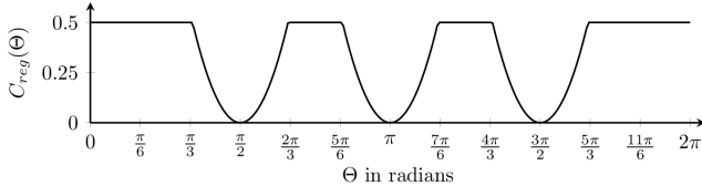
Fig. 4. C_{reg}(\Theta) when scale is 0.5 and skewness is 2.
