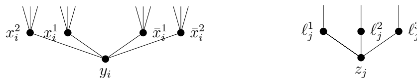
Figure 5: Variable gadget VG_i (left) and clause gadget CG_j (right).
