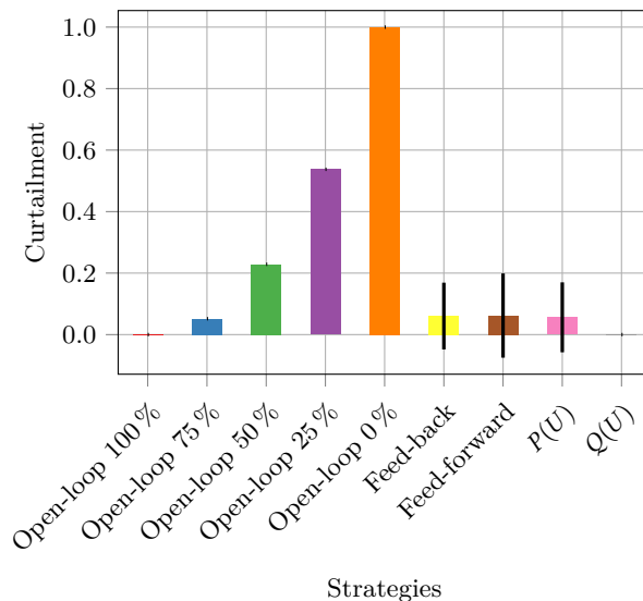
Figure 6: curtailed energy, per strategy. The coloured bar shows the mean value of lost energy across feeders and time steps. The black line shows standard deviation. Standard deviation is zero for open-loop strategies.
